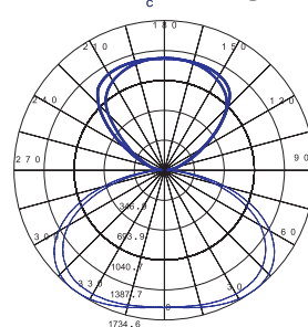
DF-015(80W,4000K,90deg/120deg)
